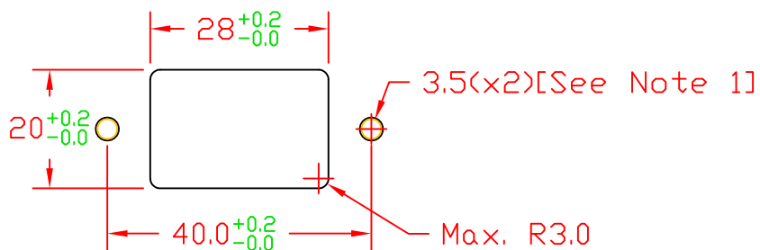
Front-side mounting
