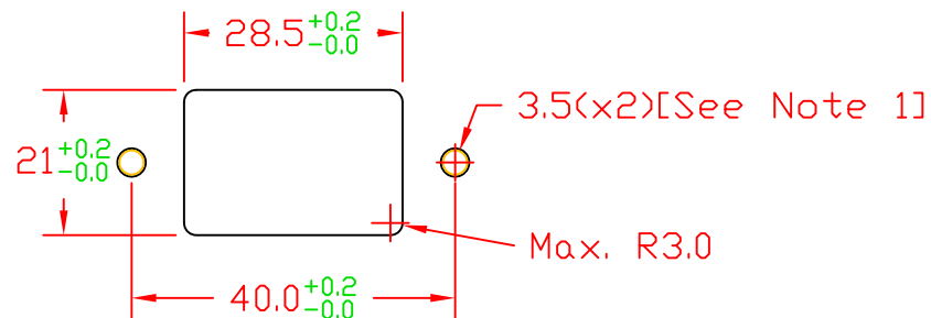
Rear-side mounting
